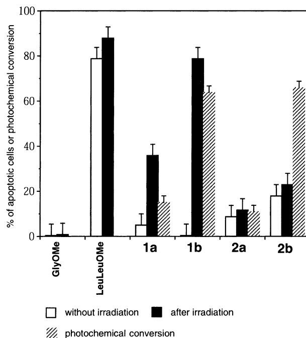
Figure 4. Induction of apoptosis (%) in HL60 cells and photochemical conversion (%) of the caged compounds. HL60 cells were treated with caged compounds according to the method described under Experimental. Without irradiation; the cells were added to GlyOMe or LeuLeuOMe or the caged compounds at 500 μM, and incubated without irradiation. After irradiation: the cells were added to GlyOMe or LeuLeuOMe or the caged compounds, and irradiated for 5 min before incubation. Photochemical conversion; the caged compounds without cells were irradiated for 5 min under the same conditions. Experiments were carried out in triplicates, and the results contained less than ±5% of standard error. The results of bioassay were shown as % of the apoptotic cells calculated from [1 - (\% \text{ of 'viable cells'}) / (\% \text{ of 'cells in control'})] . Photochemical conversion was expressed by the % of the caged compounds decreased.
