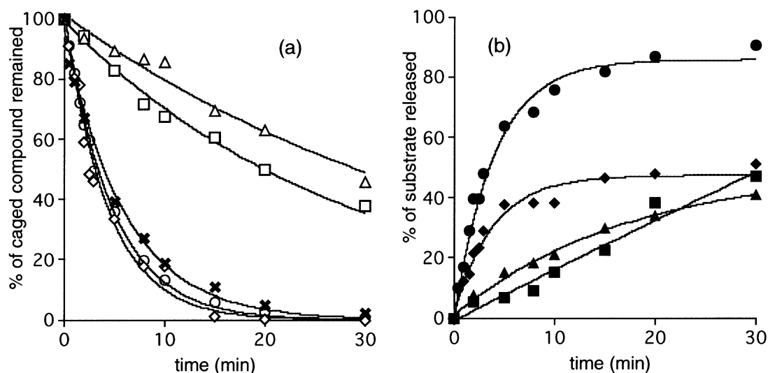
Figure 2. Photolysis of caged compounds in PBS containing 1% DMSO at 350 nm: (a) decrease of caged compounds; (b) release of LeuLeuOMe or GlyOMe (□; 1a , ○; 1b , △; 2a , ◇; 2b , ×; 3 , ■; release of LeuLeuOMe from 1a , ●; release of GlyOMe from 1b , ▲; release of GlyOMe from 2a , ◆; release of GlyOMe from 2b ).
