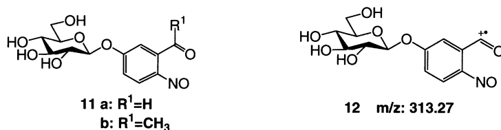
Figure 3. Structures of photolytic byproducts and the MS fragmentation product.
