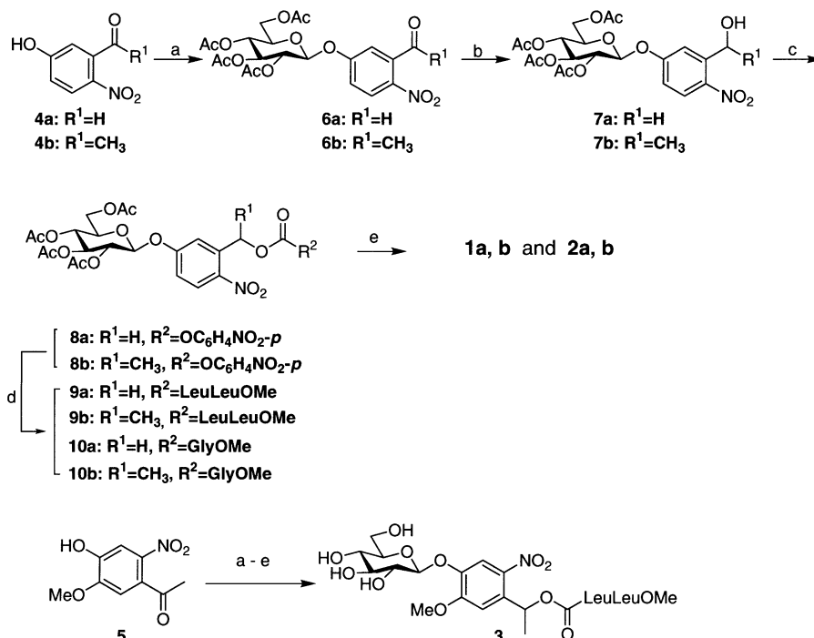
Scheme 1. Synthesis: (a) tetra- O -acetylglucopyranosyl trichloroacetimidate, BF 3 ·Et 2 O, CH 2 Cl 2 ; (b) NaBH 4 , EtOH; (c) 4-nitrophenyl chloroformate, DMAP, CHCl 3 ; (d) LeuLeuOMe·TFA, or GlyOMe·HCl, DMAP, CHCl 3 ; (e) NaOMe, MeOH.
