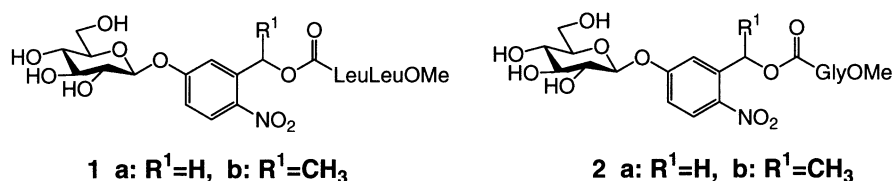
Figure 1. Structures of caged compounds.
